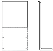
Headrest couple | Coppia poggiatesta cm 55x105h | in 21"2/3x41"1/3h
